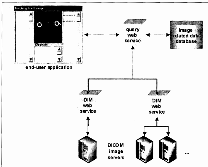
Figure 1. Collaborating Web Services for DICOM Query Management.
