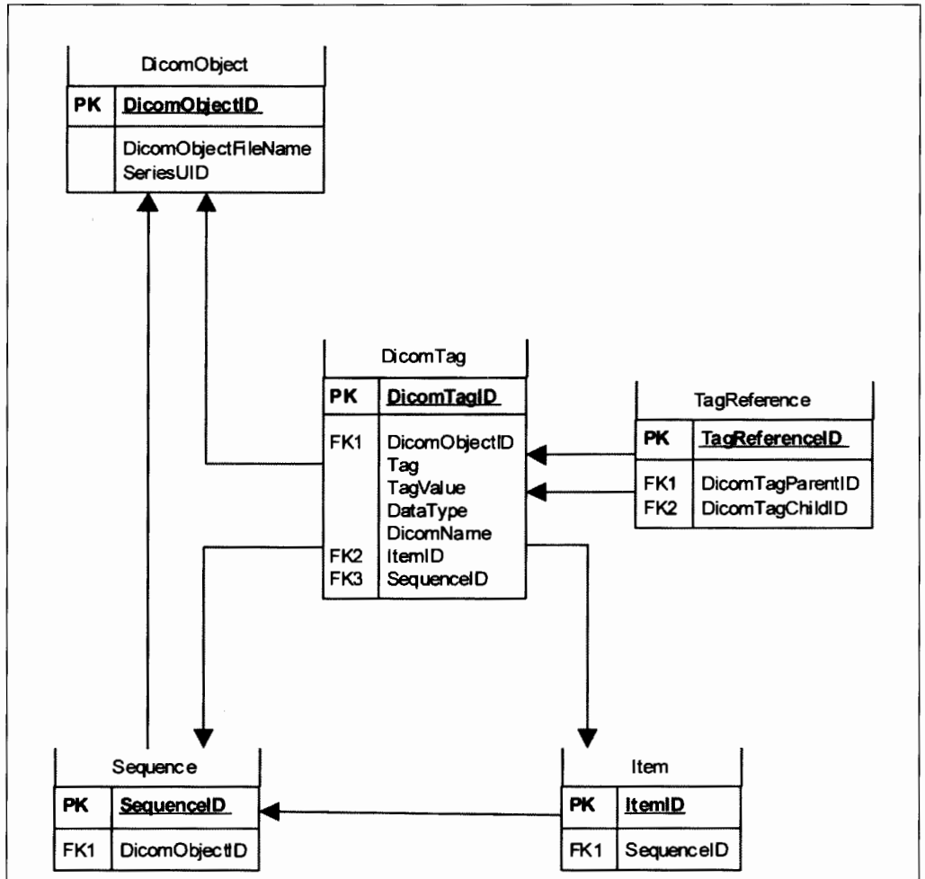
Figure 2. DICOM Attribute Database Model.
