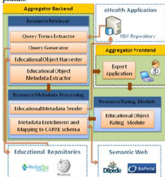
Figure 1. Component Architecture.
